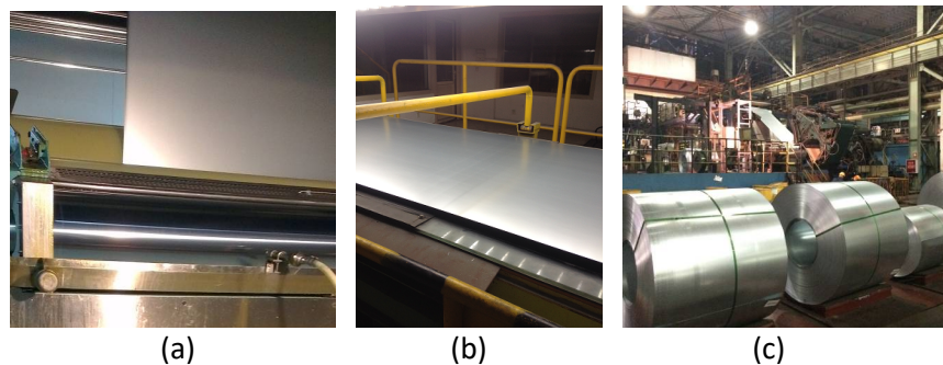
Figure 6. A line trial at Panzihua Iron and Steel Company; (a) MPT rolling-applied onto a moving galvanized steel sheet, (b) MPT-treated GI sheet after baking, and (c) MPT-treated GI coils
