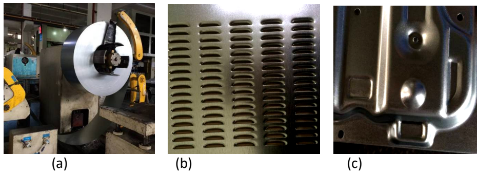
Figure 7. Formability test in a downstream client's plant (a microwave oven manufacturer); (a) uncoiling MPT-treated GI coil; (b) punched back panel and (c) stamped panel
