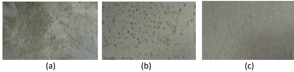
Figure 5. 3-week in-house wet stack test results for GI flat panels with different passivation treatments; (a) untreated, (b) PT-treated and (c) MPT treated (both PT and MPT film thickness was 1 \mu\text{m} )
