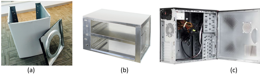
Figure 1. Applications of PMT treated galvanized steel sheets; (a) washer frame, (b) microwave oven frame and (c) a computer frame
