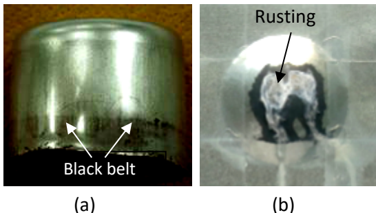
Figure 3. (a) “Black belt” occurred on a passivated galvanized steel sheet after deep drawing; (b) deformed passivated galvanized steel surface after exposed in
